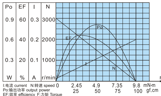
PM-33244500 特性曲线 CHARACTERISTICS
