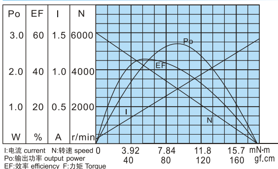
PM-33126000 特性曲线 CHARACTERISTICS
