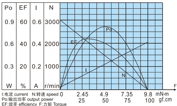
PM-33124500 特性曲线 CHARACTERISTICS
