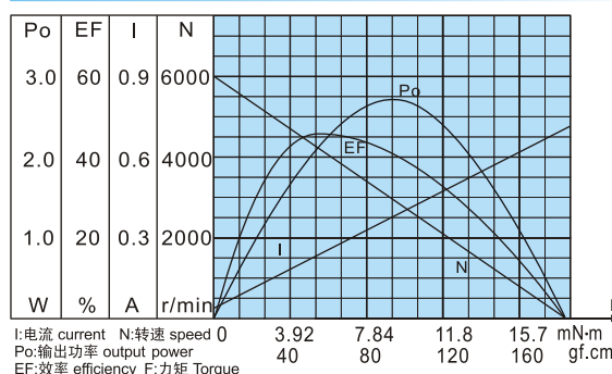
PM-33246000 特性曲线 CHARACTERISTICS
